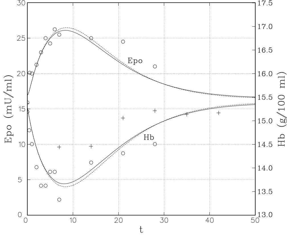
Figure 3.3: The solid curves show the age-structured model with variable velocity, while the dotted curves used V(E) = 1 , which are equivalent to the graphs in Fig. 3.1 and 3.2. The data are shown for comparison.
