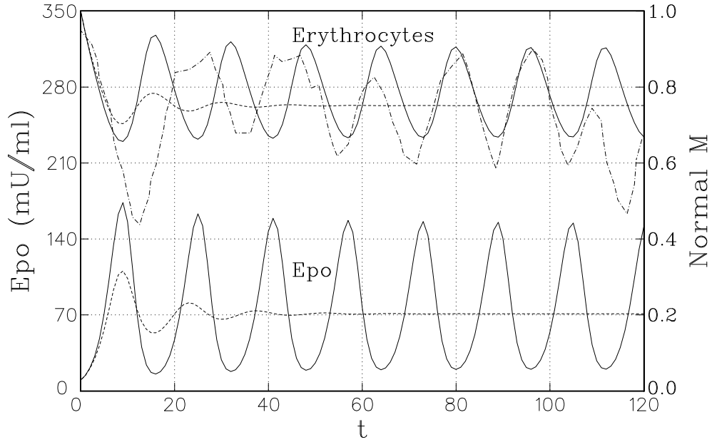
Figure 3.4: The dashed curve shows the age-structured model with variable velocity, while the solid curve used V(E) = 1 . The data from Orr et al. is shown (dot and dash curve) and has similar oscillatory behavior to the V(E) = 1 curve.
