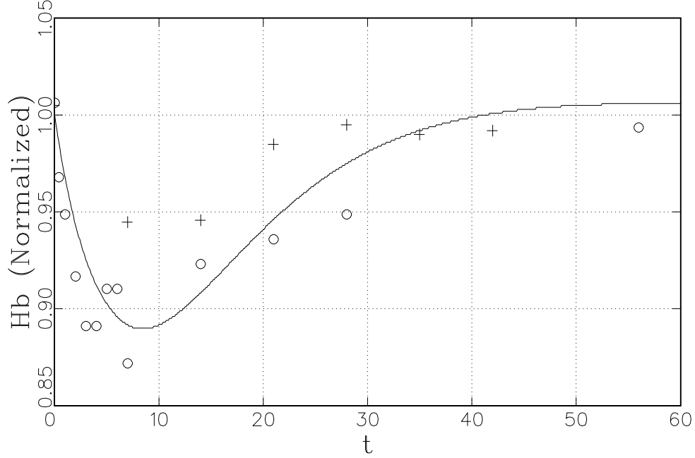
Figure 3.1: Simulation of Eqn. (2.12) with optimal parameters showing the concentration of hemoglobin following a blood donation with data of Maeda et al. (○) and Wadsworth (+).
